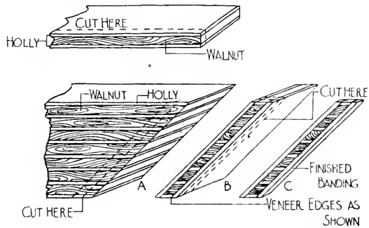
FIG. 337. STEPS IN BUILDING A BANDING.
